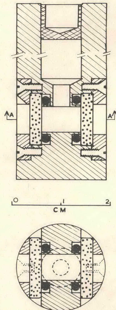
FIG. 1. High pressure optical absorption cell.
